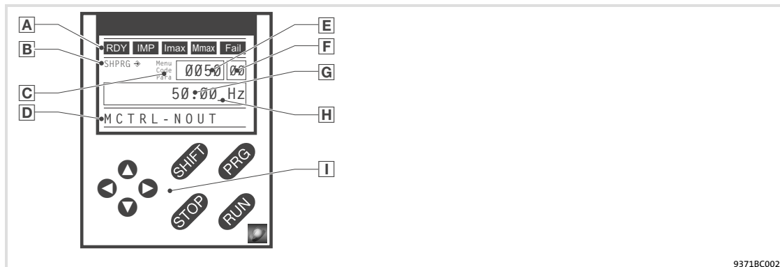
Fig. 9-4 Display elements and function keys of the XT EMZ9371BC keypad
