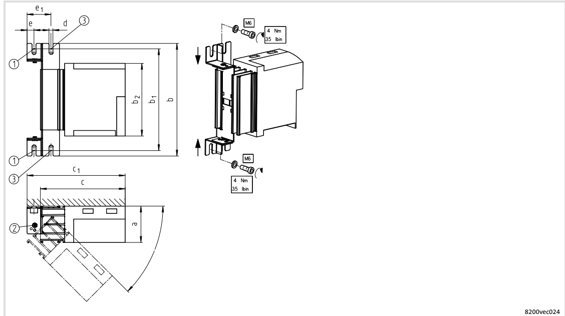
Fig. 5-9 Swivelling lateral mounting
