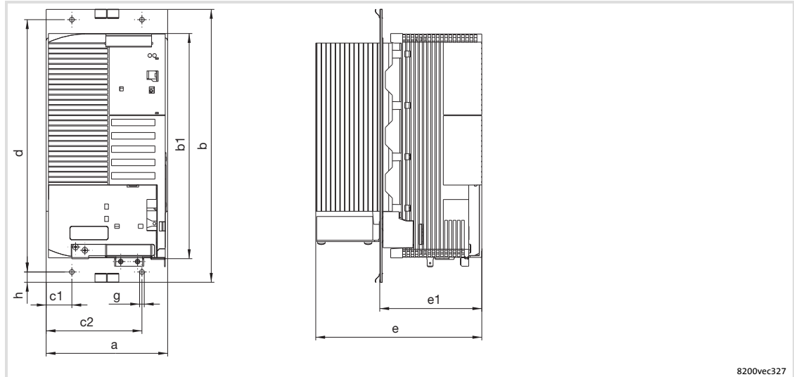
Fig. 5-11 Dimensions for thermally separated mounting 3 ... 11 kW
